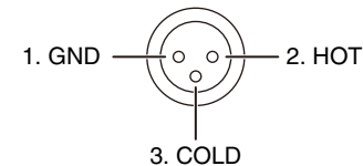
XLR output jacks
